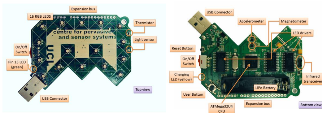
Figure 1: The top and bottom of your Engduino
